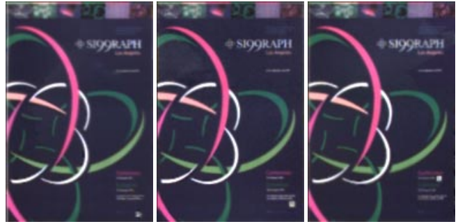
Figure 10: The diffuse albedo maps of three posters with the same texture. The posters were placed at different locations in the scene and thus received significantly different illumination. Nonetheless, the recovered albedo maps are nearly the same. For identification purposes, a small yellow square was placed in a different location on the lower right of each poster.
