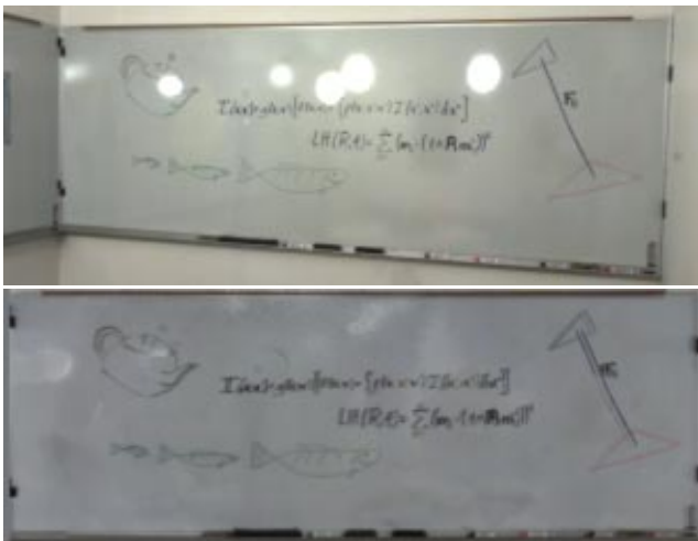
Figure 9: The top picture is a radiance image of a whiteboard, showing strong specular highlights. The bottom picture shows the diffuse albedo map of the whiteboard recovered from several images. Unlike the radiance image, the diffuse albedo map has a nearly uniform background, and is independent of the illumination.
