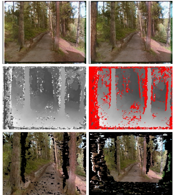
Figure 1. The Immersion '94 image-based modeling and rendering project. The top images are a stereo pair (reversed for cross-eyed stereo viewing) taken in Banff National Forest. The middle left photo is a stereo disparity map produced by John Woodfill's parallel implementation of the Zabih-Woodfill stereo algorithm [18]. To its right the map has been processed using a left-right consistency check to invalidate regions where running stereo based on the left image and stereo based on the right image did not produce consistent results. Below are two virtual views generated by casting each pixel out into space based on its computed depth estimate, and reprojecting the pixels into novel camera positions. On the left is the result of virtually moving one meter forward, on the right is the result of virtually moving one meter backward. Note the dark disoccluded areas produced by these virtual camera moves; these areas were not seen in the original stereo pair. In the Immersion '94 animations (available at http://www.debevec.org/Immersion ), these regions were automatically filled in from neighboring stereo pairs.
